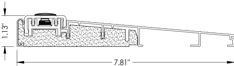
32 INSWING THRESHOLD Inswing Composite Adjustable 7-3/4\"/>
