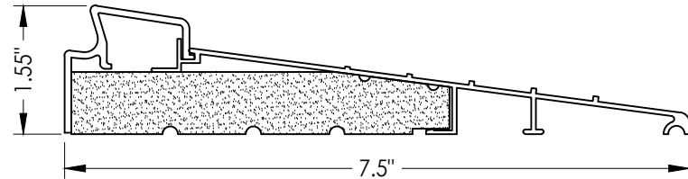
37 INSWING THRESHOLD Inswing Basic Fixed 7-1/2\"/>
