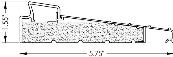
36 INSWING THRESHOLD Inswing Basic Fixed 5-3/4\"/>
